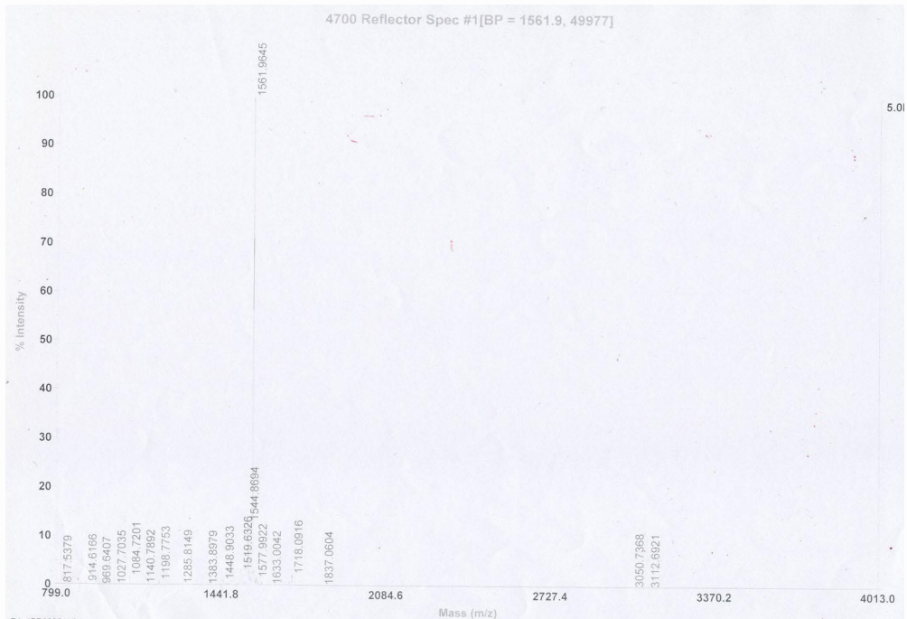
Figure 2. MASS Spectrometry
