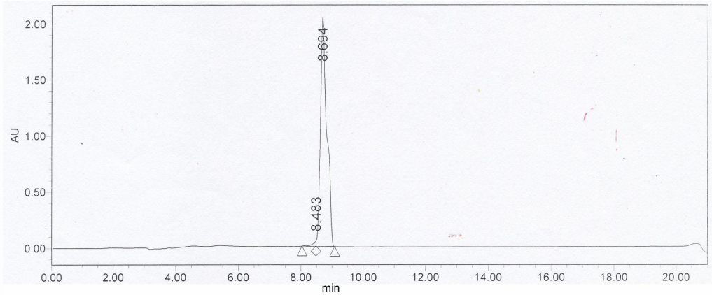
Figure 1. HPLC
