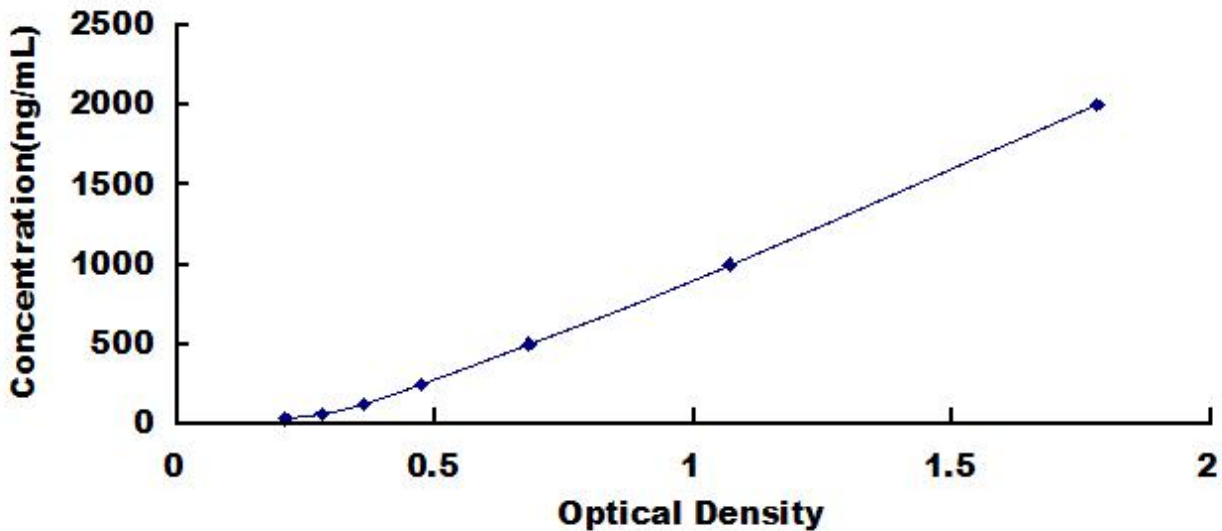
Typical Standard Curve for Glycated Albumin, Human ELISA.
