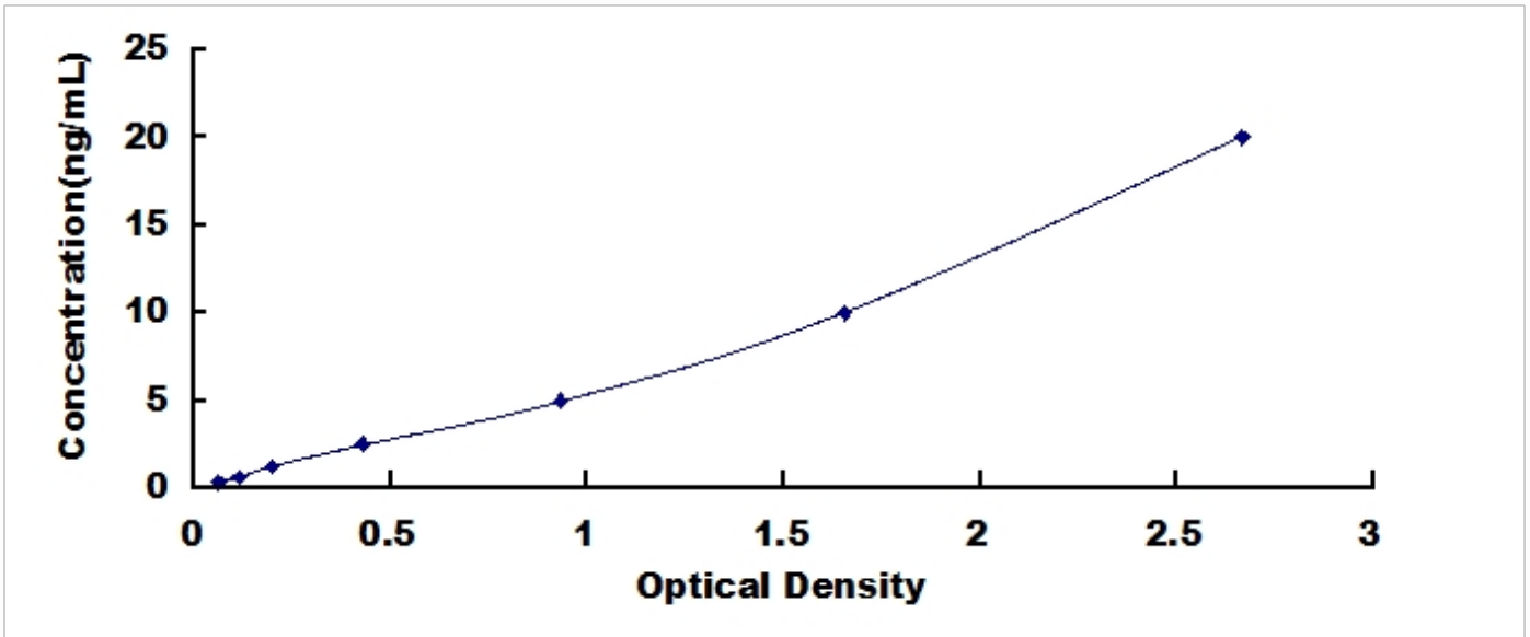
Typical Standard Curve for PDL1, Rat ELISA.
