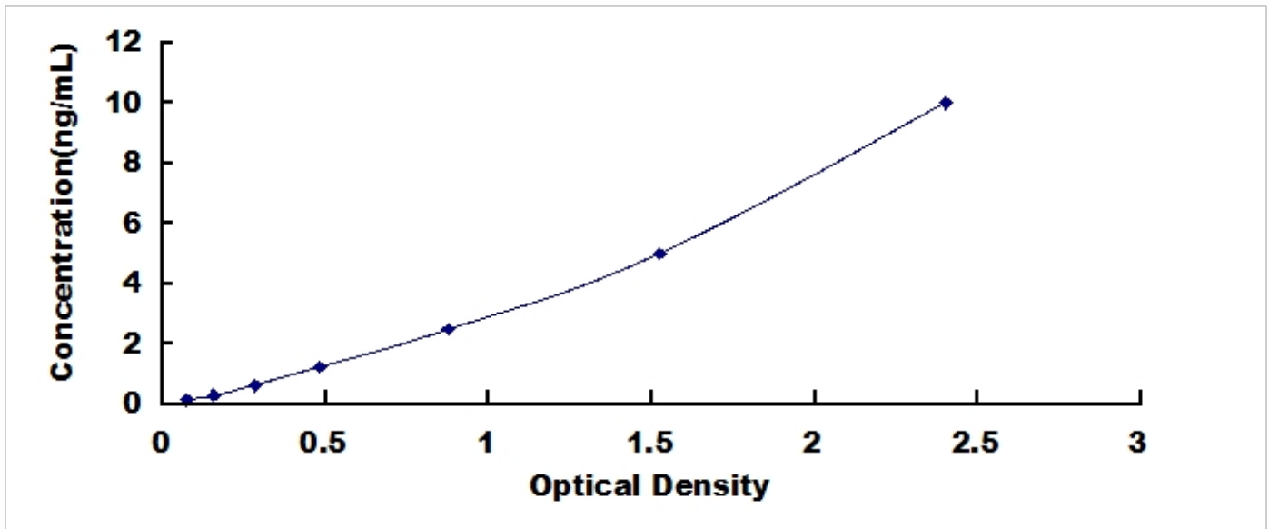
Typical Standard Curve for NSMASE, Mouse ELISA.
