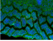
IF/ICC staining of rat intestine tissue using beta-Tubulin Mouse Monoclonal Ab.
