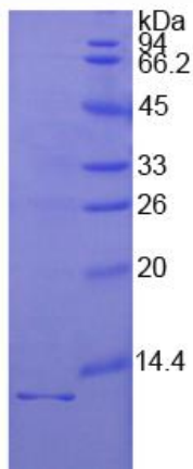
Figure 2. SDS-PAGE
