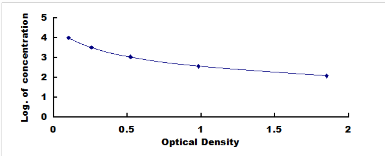
Typical Standard Curve for aMSH, Human ELISA.
