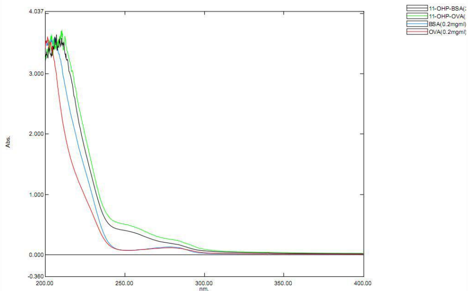
Figure 2. UV-spectrum
