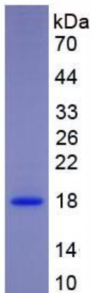
Figure 2. SDS-PAGE
