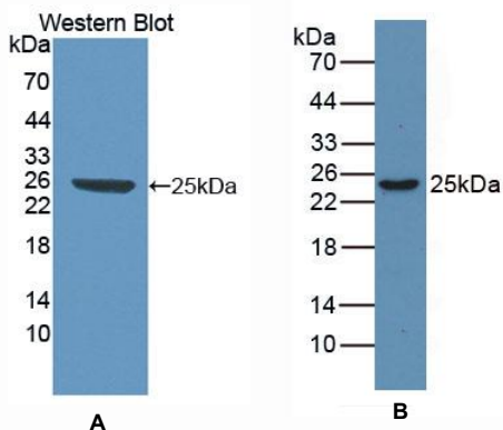
Figure 1. Western Blot
