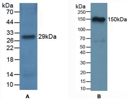
Figure 1. Western Blot
