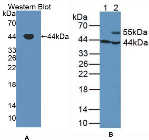
Figure 1. Western Blot
