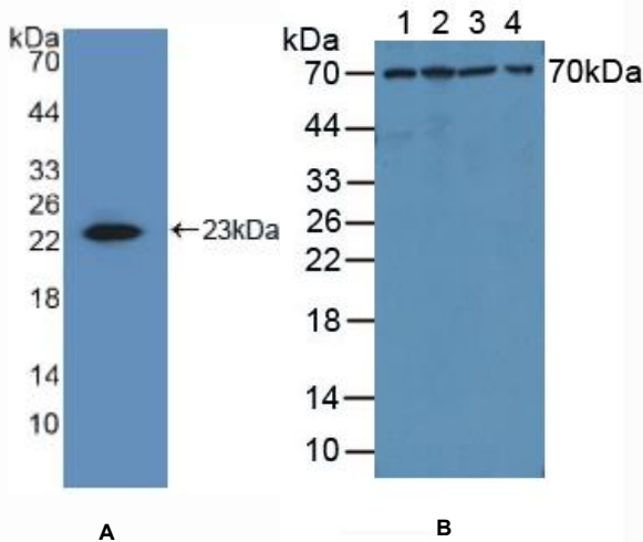
Figure 1. Western Blot
