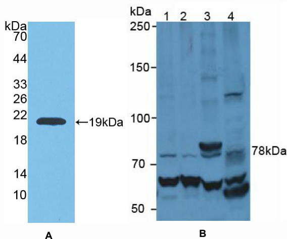
Figure 1. Western Blot
