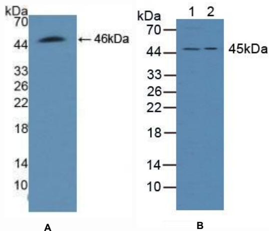
Figure 1. Western Blot
