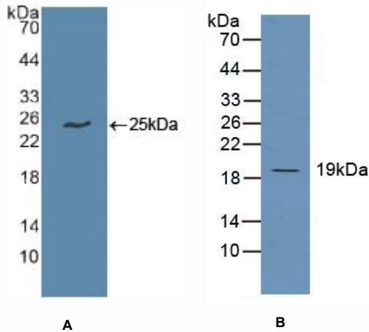
Figure 1. Western Blot
