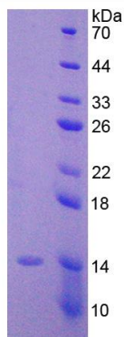
Figure 2. SDS-PAGE
