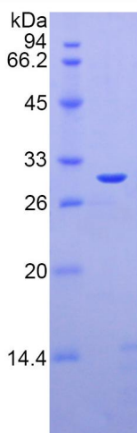
Figure 1. SDS-PAGE
