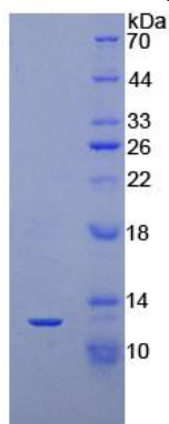
Figure 2. SDS-PAGE
