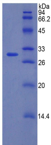
Figure 1. SDS-PAGE
