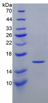
Figure 1. SDS-PAGE
