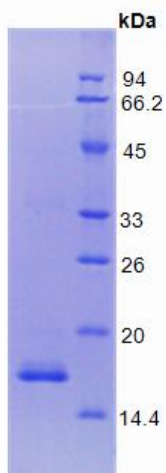
Figure 1. SDS-PAGE
