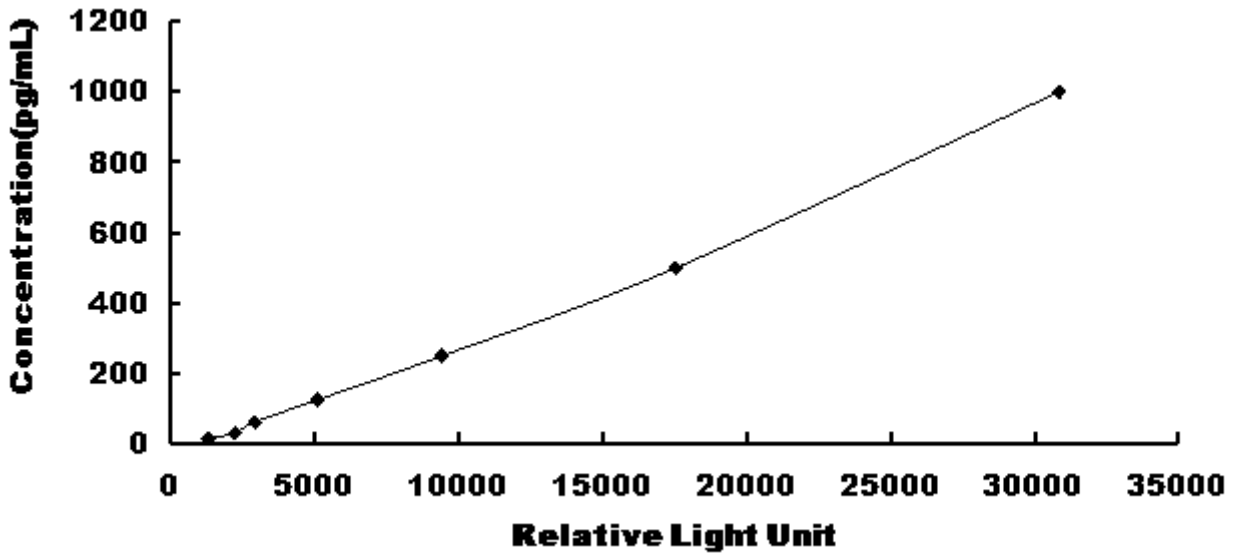
Typical Standard Curve for Equine IFNa CLIA.
