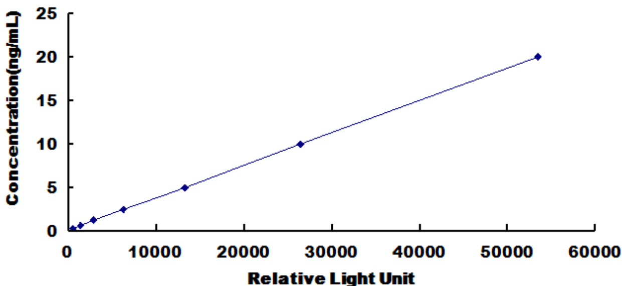
Typical Standard Curve for Human FBN1 CLIA.
