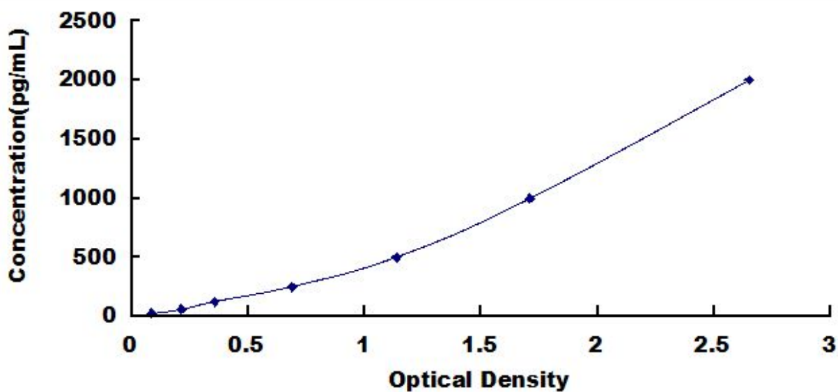
Typical Standard Curve for CTGF, Rat ELISA.
