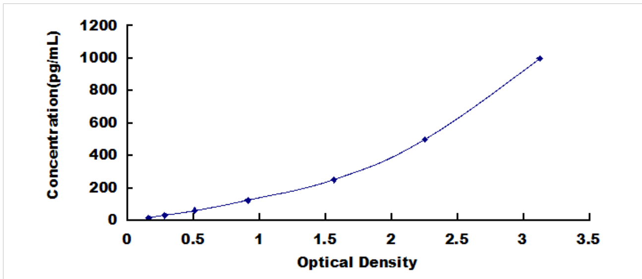
Typical Standard Curve for IL18, Cavia ELISA.
