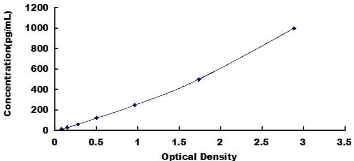
Typical Standard Curve for IL18, Rabbit ELISA.
