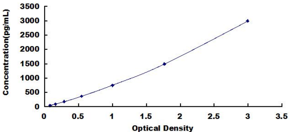
Typical Standard Curve for HMG1, Mouse ELISA.
