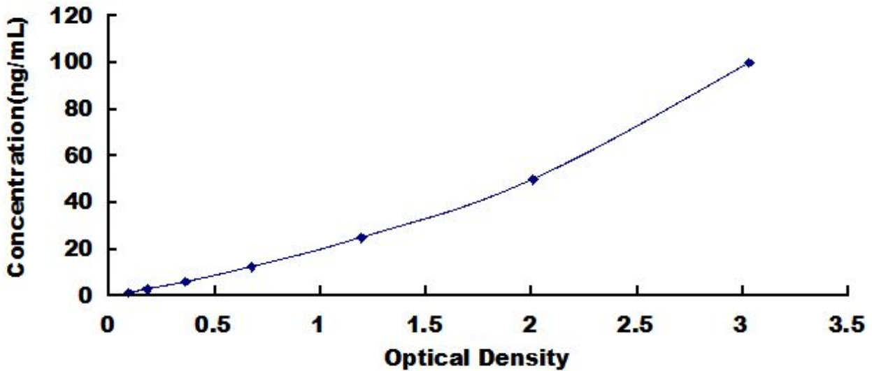
Typical Standard Curve for IgM, Gallus ELISA.
