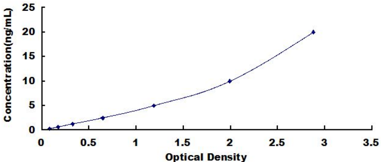
Typical Standard Curve for ICAM1, Mouse ELISA.
