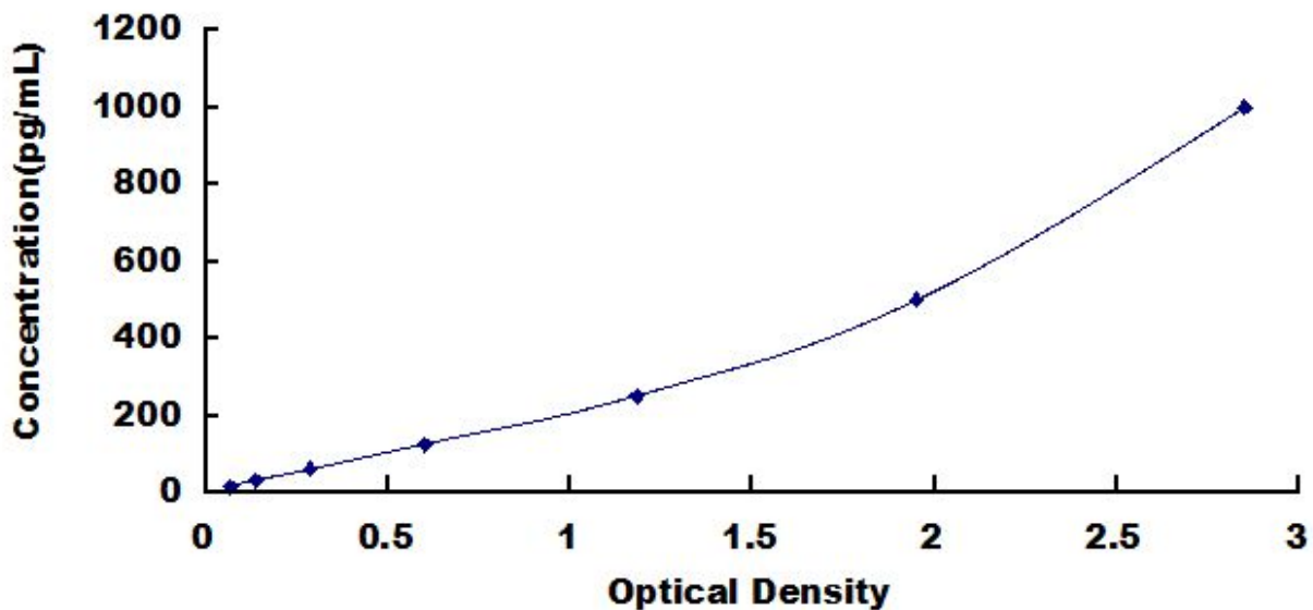
Typical Standard Curve for AQP9, Human ELISA.
