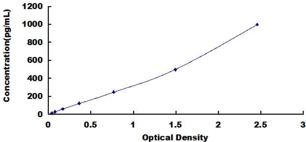
Typical Standard Curve for BMP1, Human ELISA.
