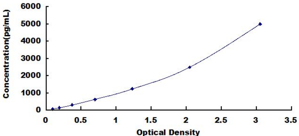
Typical Standard Curve for BMP1, Mouse ELISA.
