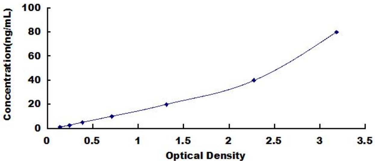
Typical Standard Curve for CYPA, Human ELISA.
