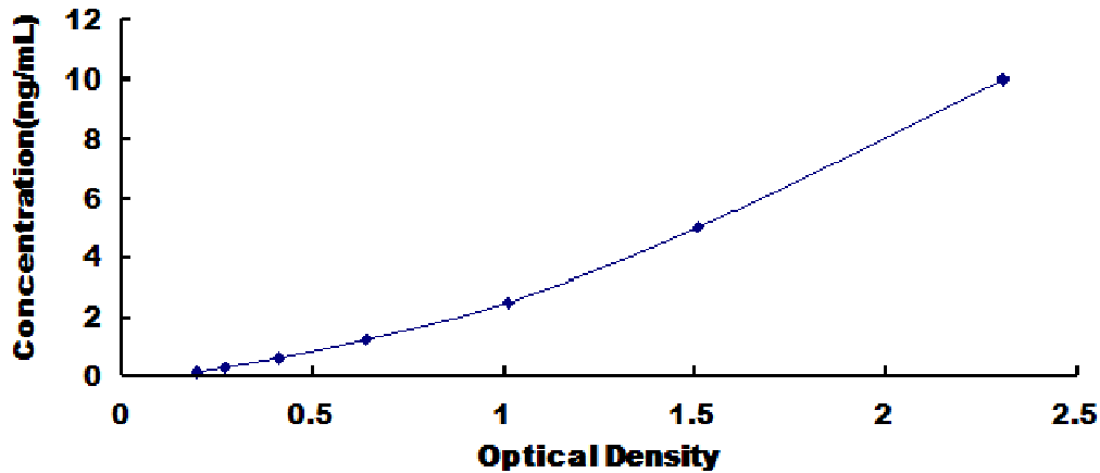
Typical Standard Curve for b3GAT1, Human ELISA.
