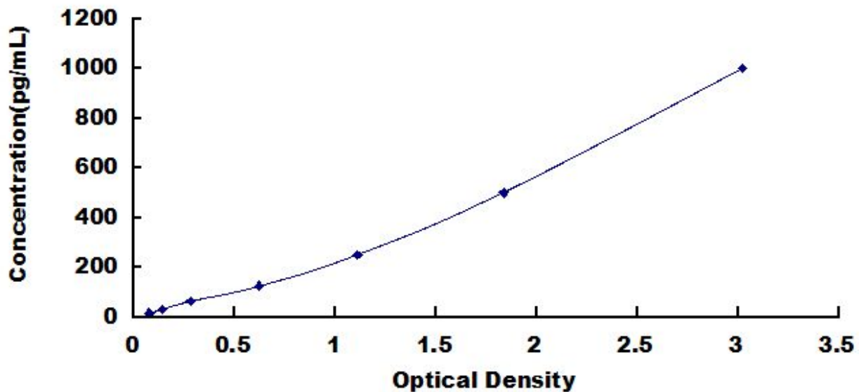
Typical Standard Curve for HBEGF, Mouse ELISA.
