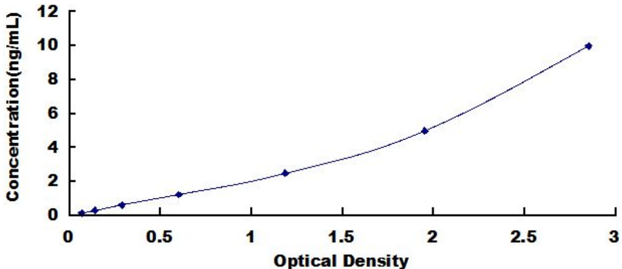
Typical Standard Curve for CFI, Human ELISA.
