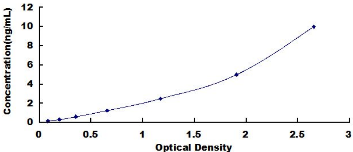
Typical Standard Curve for COL6a1, Rat ELISA.
