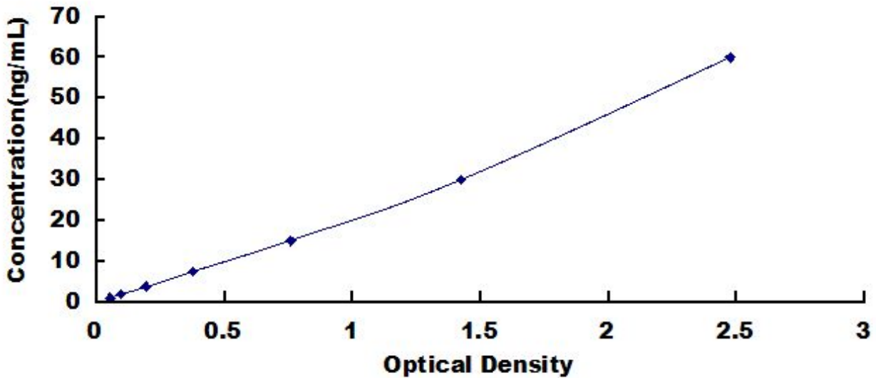
Typical Standard Curve for Antithrombin, Mouse ELISA.
