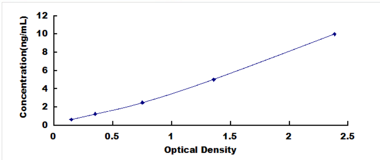
Typical Standard Curve for DHODH, Human ELISA.
